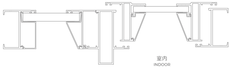
室外 OUTDOOR
