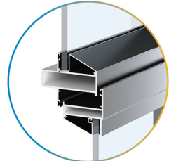
外压线制作 SLOPING GLAZING STOP
