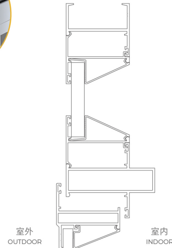
外压线制作 SLOPING GLAZING STOP
