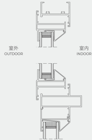
70/50 转换图 STRENGTHEN THE CENTER COLUMN
