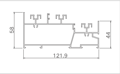
Model: XJ-FTLC12503 ( slide down ) Thickness: 1.3mm Weight: 2.066kg/m
