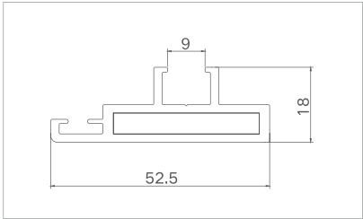
Model: XJ-TDM105228A ( hook ) Thickness: 2.0mm Weight: 0.716kg/m
