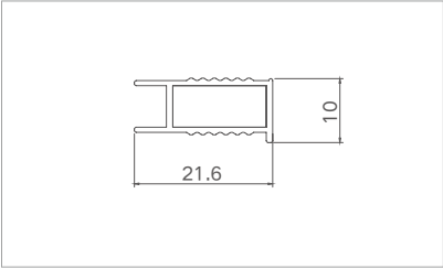
Model: PKM40426 ( Reverse cover ) Thickness: 1.0mm Weight: 0.146kg/m
