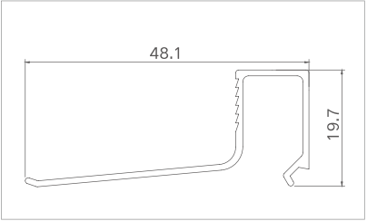
Model: XJ-PKC5030 (Solid double glass bead) Thickness: 1.0mm Weight: 0.24kg/m
