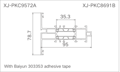
Model: XJ-DQPK9572 ( Middle column ) Thickness: 1.75mm Weight: 1.949kg/m
