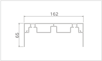
Model: XJ-TDM16229 ( Triple-linkage upper rail ) Thickness: 1.4mm Weight: 2.274kg/m
