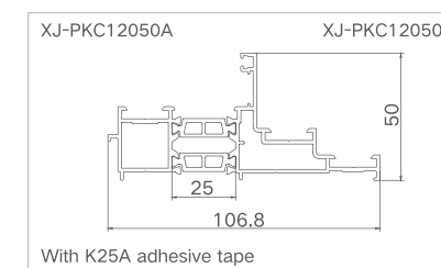
Model: XJ-DQPK12050 ( Attached frame )
