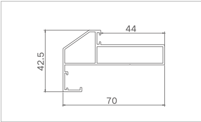
Model: XJ-PKM40437 ( front door casing ) Thickness: 1.2mm Weight: 0.782kg/m
