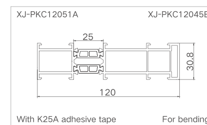
Model: XJ-DQPK12051 ( Outer frame )
