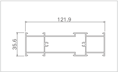
Model: XJ-FTLC12504 ( middle column ) Thickness: 1.3mm Weight: 1.499kg/m
