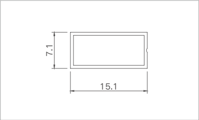
Model: XJ-XL008 ( Grid strip ) Thickness: 0.6mm Weight: 0.069kg/m
