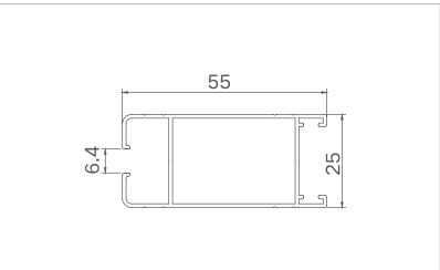
Model: XJ-TLC8009 Thickness: 1.0mm Weight: 0.492kg/m
