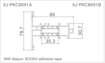
Model: XJ-DQPK8691 ( Middle column ) Thickness: 1.75mm Weight: 1.816kg/m
