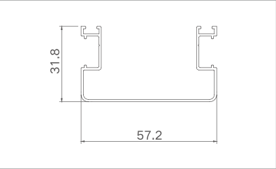
Model: XJ-ZTDM10619B ( 70 double hook ) Thickness: 1.0mm Weight: 0.433kg/m
