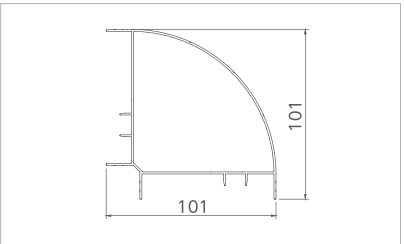
Model: XJ-TLC8013 Thickness: 1.2mm Weight: 1.249kg/m
