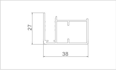
Model: XJ-MTX3801 ( Door pocket line ) Thickness: 1.2mm Weight: 0.443kg/m
