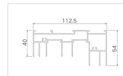
Model: XJ-FTLC11502 ( Slide up )
