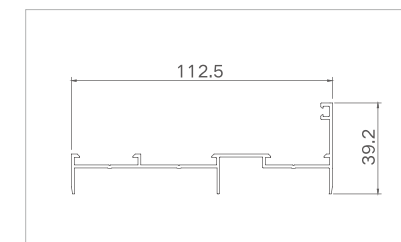
Model: XJ-FTLC11505 (waist cover plate)
