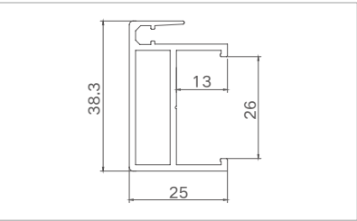
Model: XJ-FTLC12506 ( Hook ) Thickness: 1.6mm Weight: 0.556kg/m
