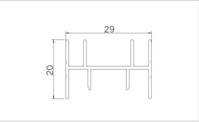
Model: XJ-TLC8012 Thickness: 1.0mm Weight: 0.265kg/m
