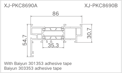
Model: XJ-DQPK9571 ( Outer frame ) Thickness: 1.75mm Weight: 1.647kg/m
