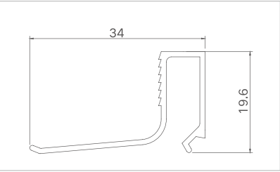
Model: XJ-PKC5024 (Double glass sash bead) Thickness: 1.0mm Weight: 0.21kg/m
