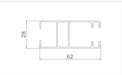
Model: XJ-TLC8038 Thickness: 1.1mm Weight: 0.68kg/m
