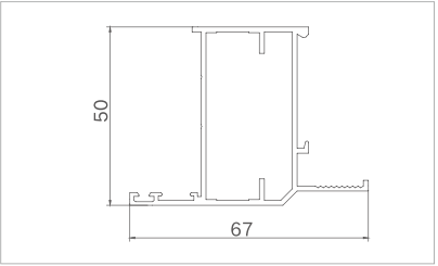
Model: XJ-PKC5021 (Glass sash) Thickness: 1.4mm Weight: 0.84kg/m
