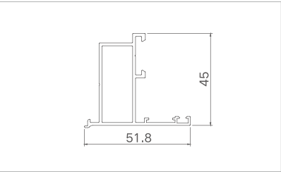
Model: XJ-PKC5011 ( Conversion material ) Thickness: 1.4mm Weight: 0.664kg/m
