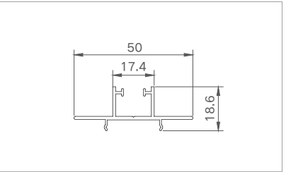
Model: XJ-DZ12007 ( close ) Thickness: 1.3mm Weight: 0.318kg/m
