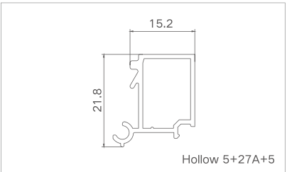
Model: XJ-PKC9578 ( Bead ) Thickness: 1.0mm Weight: 0.216kg/m
