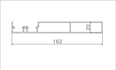
Model: XJ-TDM16220 Thickness: 1.4mm Weight: 1.48kg/m
