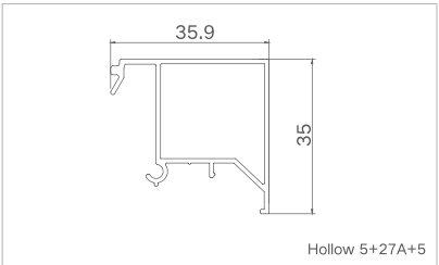
Model: XJ-PKC8695 ( Solid glass bead ) Thickness: 1.0mm Weight: 0.38kg/m
