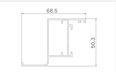
Model: XJ-FPKC4006 ( Yarn sash ) Thickness: 1.1mm Weight: 0.691kg/m
