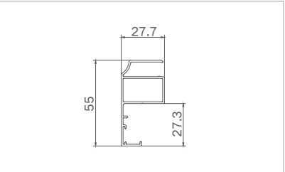
Model: XJ-PKM40203 ( front double door casing ) Thickness: 1.15mm Weight: 0.523kg/m
