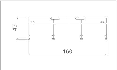
Model: XJ-ZTDM16007 ( three-track upper sliding ) Thickness: 1.2mm Weight: 1.814kg/m
