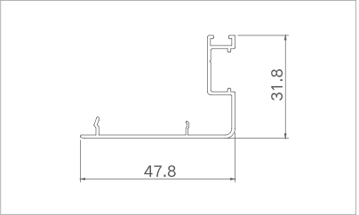
Model: XJ-ZTDM10605A ( 70 single hook ) Thickness: 1.0mm Weight: 0.289kg/m
