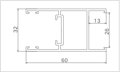
Model: XJ-FTLC12508 ( upper and lower part ) Thickness: 1.4mm Weight: 0.788kg/m
