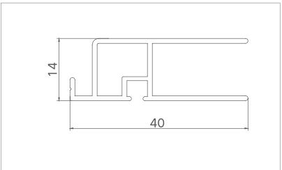
Model: XJ-TLC8040 Thickness: 1.1mm Weight: 0.32kg/m
