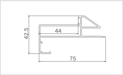
Model: XJ-PKM40438 ( Back double door casing ) Thickness: 1.2mm Weight: 0.814kg/m
