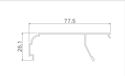
Model: XJ-TLC11509 ( circular arc bead ) Thickness: 1.1mm Weight: 0.403kg/m
