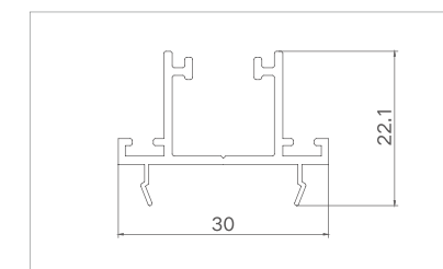
Model: XJ-TLC11506C ( Glass sash closing )
