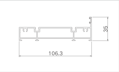
Model: XJ-ZTDM10603 ( high double rail ) Thickness: 1.4mm Weight: 1.24kg/m
