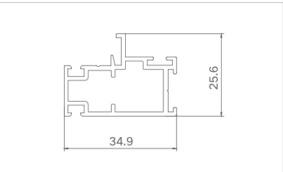
Model: XJ-PKC9575 ( Yarn sash ) Thickness: 1.3mm Weight: 0.474kg/m
