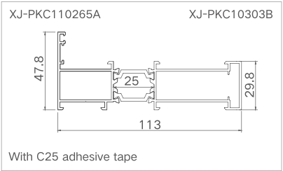
Model: XJ-DQPK110265 ( Outer frame ) Thickness: 1.3mm Weight: 1.517kg/m
