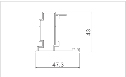
Model: XJ-FPKC4007 ( Frame ) Thickness: 1.2mm Weight: 0.632kg/m
