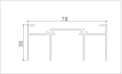
Model: XJ-TLC8002 Thickness: 1.1mm Weight: 0.701kg/m
