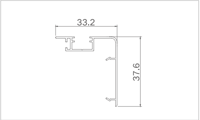
Model: XJ-TLC11506A ( glass sash hook ) Thickness: 0.85mm Weight: 0.236kg/m
