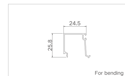
Model: XJ-PKC8509 ( Square bead )
