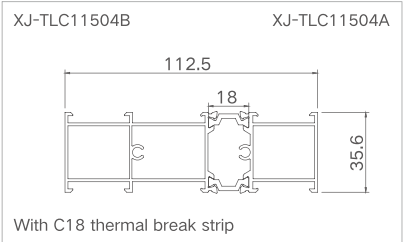
Model: XJ-DQTLC11504 ( Middle column ) Thickness: 1.3mm Weight: 1.709kg/m
