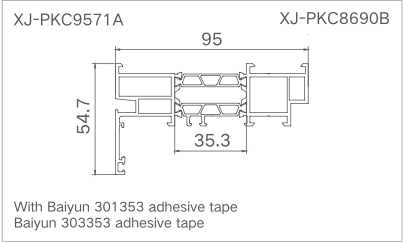
Model: XJ-DQPK9571 ( Outer frame ) Thickness: 1.75mm Weight: 1.789kg/m
