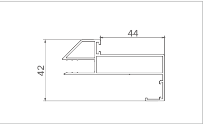
Model: XJ-PKM40436 ( back door casing ) Thickness: 1.2mm Weight: 0.808kg/m
