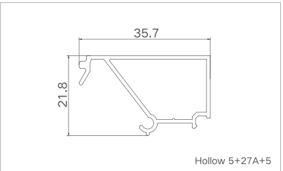
Model: XJ-PKC8696 ( Glass sash bead ) Thickness: 1.0mm Weight: 0.29kg/m
