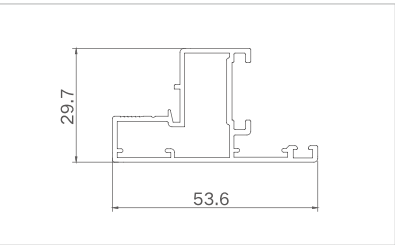
Model: XJ-FPKC6503 ( Yarn sash ) Thickness: 1.2mm Weight: 0.594kg/m
