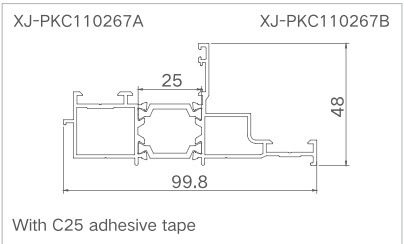
Model: XJ-DQPK110267 ( Attached frame ) Thickness: 1.3mm Weight: 1.302kg/m
