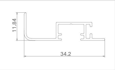
Model: XJ-TLC11506B ( double-color hook ) Thickness: 0.85mm Weight: 0.158kg/m
