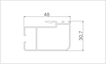
Model: XJ-TLC8010 Thickness: 1.0mm Weight: 0.507kg/m
