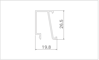
Model: XJ-PKC5012 ( Bead ) Thickness: 1.0mm Weight: 0.208kg/m
