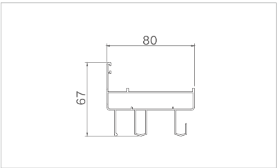
Model: XJ-TLC8037 Thickness: 1.2mm Weight: 1.17kg/m
