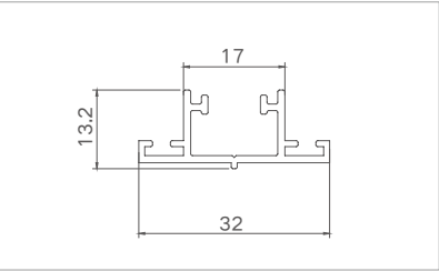
Model: XJ-FTLC12509 ( lock slots ) Thickness: 1.2mm Weight: 0.267kg/m
