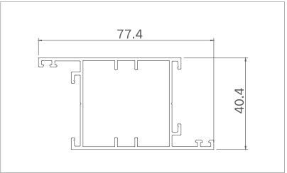
Model: XJ-FPKC4002 ( Glass sash ) Thickness: 1.2mm Weight: 0.862kg/m
