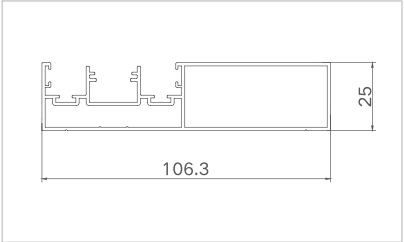
Model: XJ-ZTDM10617 ( Frame ) Thickness: 1.2mm Weight: 1.107kg/m
