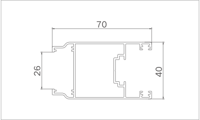
Model: XJ-TDM105166 ( Glass sash ) Thickness: 1.2mm Weight: 0.892kg/m
