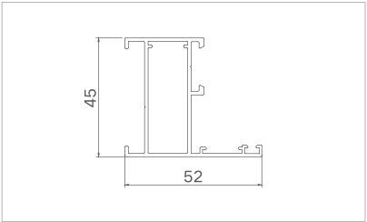
Model: XJ-PKC5009 ( Frame ) Thickness: 1.35mm Weight: 0.713kg/m
