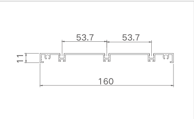
Model: J-ZTDM16008 ( three-rail ) Thickness: 1.4mm Weight: 0.991kg/m
