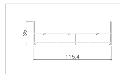
Model: XJ-FTLC11501 ( Edge seal )
