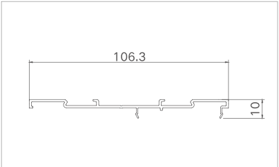
Model: XJ-ZTDM10613 ( frame cover plate ) Thickness: 1.2mm Weight: 0.470kg/m
