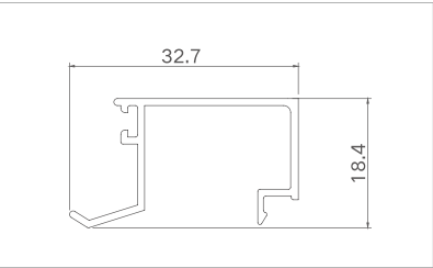
Model: XJ-FPKC4003 ( Bead ) Thickness: 1.0mm Weight: 0.216kg/m
