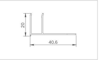
Model: XJ-TDM11083A ( Upper rail F groove ) Thickness: 1.0mm Weight: 0.211kg/m
