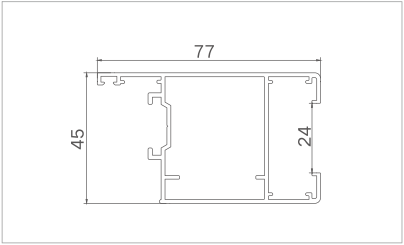
型号: XJ-FPKC9503 ( Gauze bead ) Thickness: 1.35mm Weight: 1.019kg/m
