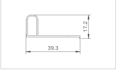
Model: XJ-TDM11083B ( Upper rail P groove ) Thickness: 1.0mm Weight: 0.196kg/m
