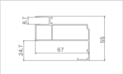
Model: XJ-PKM40453 ( Back double door casing ) Thickness: 1.15mm Weight: 0.792kg/m
