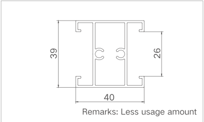
Model: XJ-ZTDM10609 ( Middle horizontal for glass sash ) Thickness: 1.2mm Weight: 0.708kg/m
