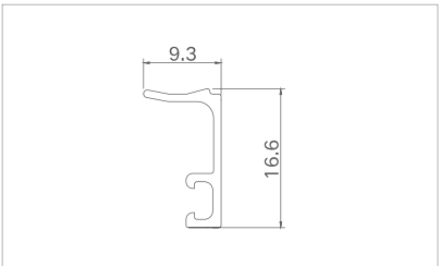
Model: XJ-PKC12552A ( Gauze bead ) Thickness: 0.9mm Weight: 0.089kg/m
