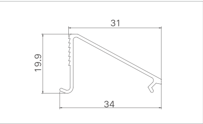
Model: XJ-PKC5023 (Single glass sash bead) Thickness: 1.0mm Weight: 0.18kg/m
