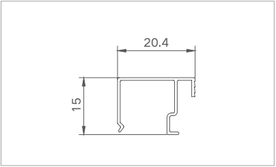
Model: XJ-TDM9038 ( Bead ) Thickness: 0.7 mm Weight: 0.111kg/m
