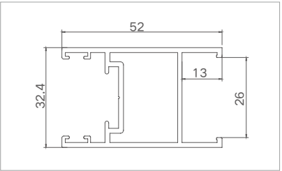
Model: XJ-FTLC12505 ( Glass sash ) Thickness: 1.6mm Weight: 0.794kg/m
