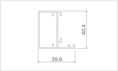
Model: XJ-FPKC4001 ( Outer frame ) Thickness: 1.2mm Weight: 0.558kg/m
