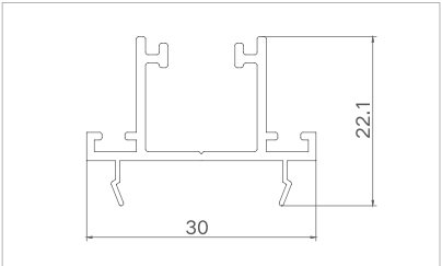
Model: XJ-TLC11506C ( Glass sash closing ) Thickness: 1.2mm Weight: 0.274kg/m
