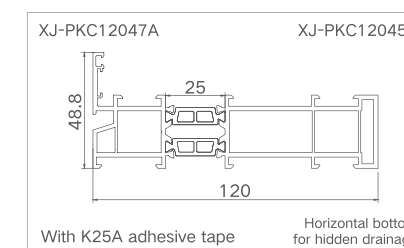
Model: XJ-DQPK12047 ( Outer frame )
