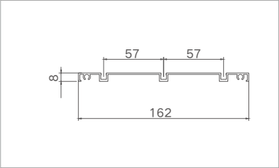
Model: XJ-TDM16203 (Triple-linkage lower rail ) Thickness: 1.35mm Weight: 0.905kg/m
