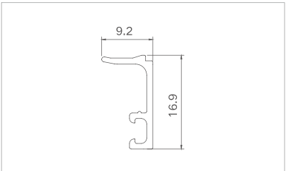
Model: XJ-PKC12552A ( Gauze bead ) Thickness: 1.1mm Weight: 0.095kg/m
