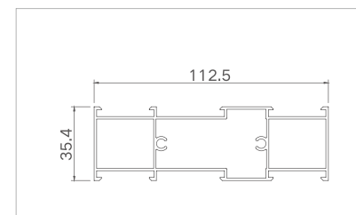
Model: XJ-FTLC11504 ( middle column )
