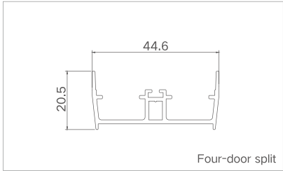
Model: XJ-TDM105233A ( close ) Thickness: 1.4mm Weight: 0.409kg/m
