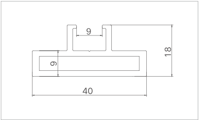
Model: TDM105227 ( Glass sash ) Thickness: 2.0mm Weight: 0.611kg/m
