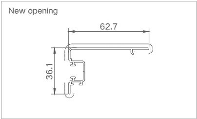
Model: XJ-DT13208C ( Single hook ) Thickness: 1.2mm Weight: 0.455kg/m
