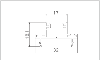
Model: XJ-FTLC12510 ( close ) Thickness: 1.2mm Weight: 0.26kg/m
