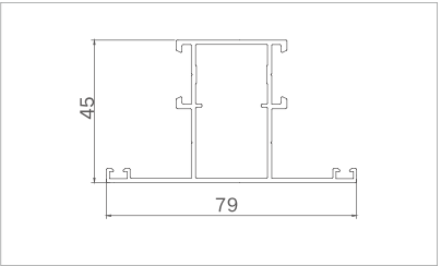
Model: XJ-PKC5010 ( Middle column ) Thickness: 1.35mm Weight: 0.869kg/m
