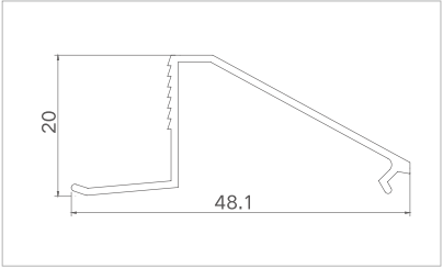
Model: XJ-PKC5022 (Solid single glass bead) Thickness: 1.0mm Weight: 0.22kg/m
