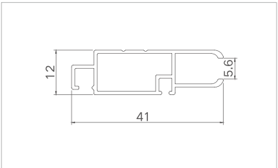
Model: XJ-TLC8015 Thickness: 0.9mm Weight: 0.273kg/m
