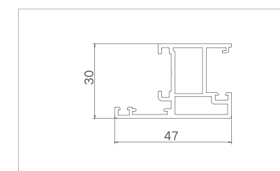
Model: XJ-PKC12805 ( Yarn sash )
