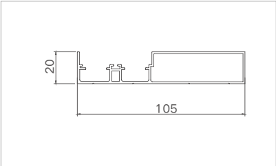
Model: XJ-TDM105222 Thickness: 1.2mm Weight: 0.898kg/m
