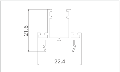
Model: XJ-TLC11507C ( yarn sash closing ) Thickness: 1.2mm Weight: 0.226kg/m
