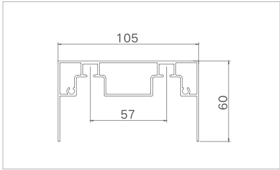
Model: XJ-TDM105230 ( Upper rail ) Thickness: 1.4mm Weight: 1.648kg/m
