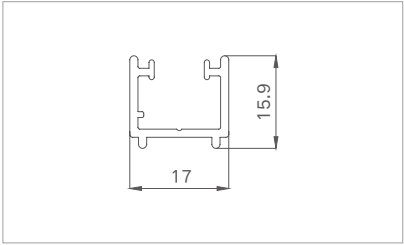
Model: XJ-TDM9039-A ( lock slots ) Thickness: 1.4mm Weight: 0.206kg/m
