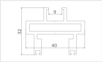
Model: TDM105229 ( Up and down horizontal ) Thickness: 2.0mm Weight: 0.902kg/m
