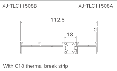
Model: XJ-DQTLC11508 Thickness: 1.4mm Weight: 1.045kg/m
