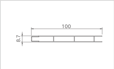
Model: XJ-KB007 ( Buckle plate ) Thickness: 0.07mm Weight: 0.44kg/m
