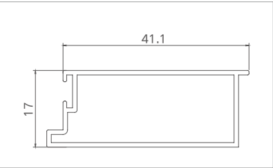
Model: XJ-FTLC12512 ( side seal cover plate ) Thickness: 1.0mm Weight: 0.312kg/m
