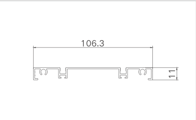
Model: XJ-ZTDM10616 ( track rail ) Thickness: 1.2mm Weight: 1.637kg/m
