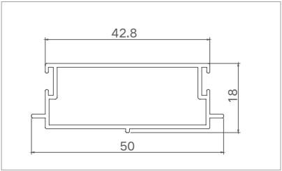
Model: XJ-FTLC12513 ( side seal cover plate ) Thickness: 1.0mm Weight: 0.36kg/m
