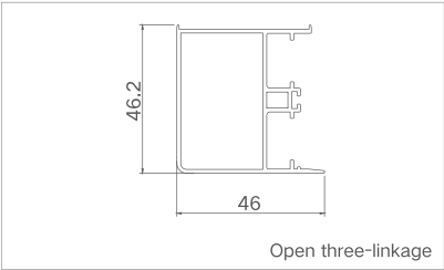
Model: XJ-TDM105235 ( Corner angle ) Thickness: 1.2mm Weight: 0.740kg/m
