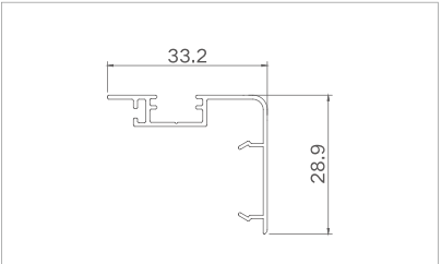
Model: XJ-TLC11507A ( yarn sash hook ) Thickness: 0.85mm Weight: 0.209kg/m
