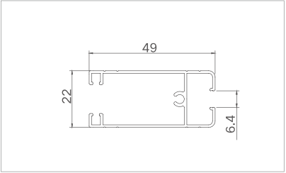
Model: XJ-TLC8011 Thickness: 1.0mm Weight: 0.436kg/m
