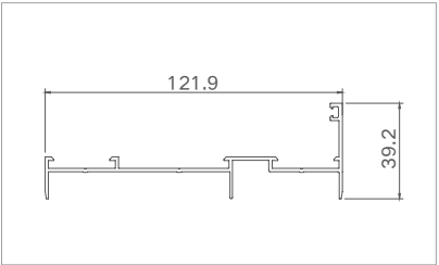
Model: XJ-FTLC12511 ( waist cover plate ) Thickness: 1.4mm Weight: 0.814kg/m
