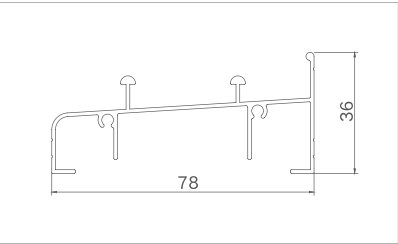
Model: XJ-TLC8004 Thickness: 1.1mm Weight: 0.636kg/m
