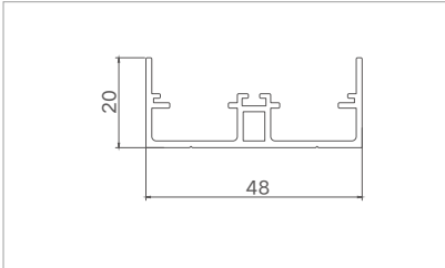
Model: XJ-TDM105234 ( Single side sealing ) Thickness: 1.3mm Weight: 0.475kg/m
