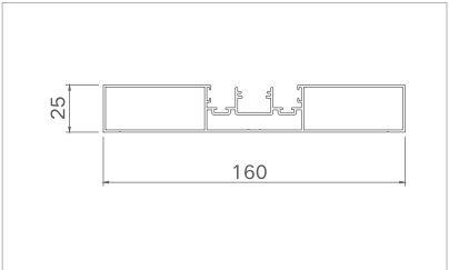
Model: XJ-ZTDM16005 ( three-rail frame ) Thickness: 1.2mm Weight: 1.509kg/m
