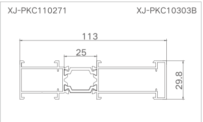
Model: XJ-DQPK110271 ( Outer frame ) Thickness: 1.3mm Weight: 1.448kg/m
