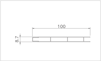
Model: XJ-KB007 ( Buckle plate ) Thickness: 0.7mm Weight: 0.44kg/m
