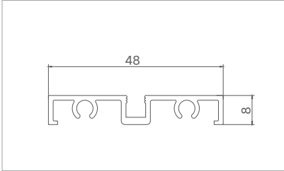
Model: XJ-TDM105240 ( Single rail ) Thickness: 1.3mm Weight: 0.357kg/m
