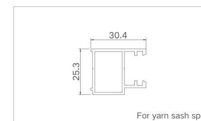
Model: XJ-PKC11076 ( False middle yarn )
