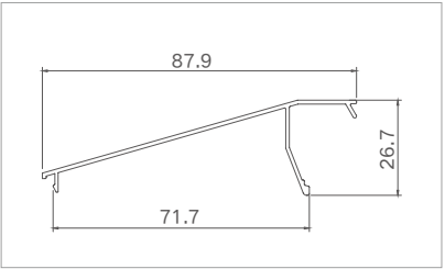
Model: XJ-FTLC12514 ( bead for the bevel edge ) Thickness: 1.1mm Weight: 0.377kg/m
