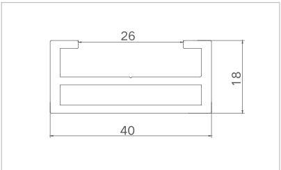
Model: PKM40429 ( Glass sash ) Thickness: 2.0mm Weight: 0.676kg/m
