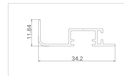
Model: XJ-TLC11506B ( double-color hook )
