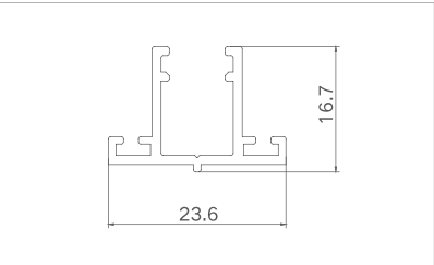
Model: XJ-TLC11510 ( yarn sash lock slot ) Thickness: 1.2mm Weight: 0.218kg/m
