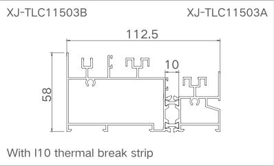
Model: XJ-DQTLC11503 ( slide down ) Thickness: 1.3mm Weight: 2.265kg/m
