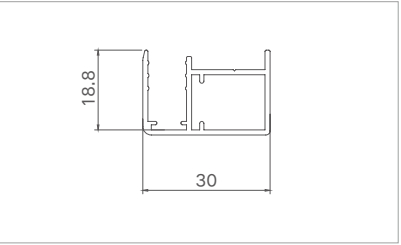
Model: XJ-PKM40435 ( front double door casing ) Thickness: 1.2mm Weight: 0.351kg/m
