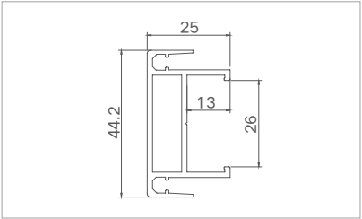
Model: XJ-FTLC12507 ( smooth double hook ) Thickness: 1.6mm Weight: 0.633kg/m
