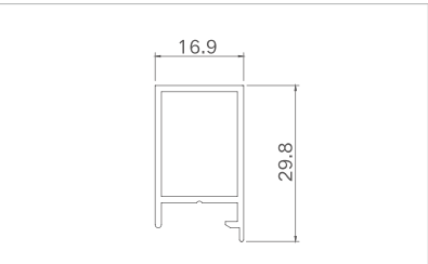
Model: XJ-PKC10028 ( Lattice base ) Thickness: 1.2mm Weight: 0.283kg/m
