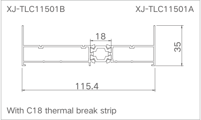
Model: XJ-DQTLC11501 ( Outer frame ) Thickness: 1.3mm Weight: 1.254kg/m
