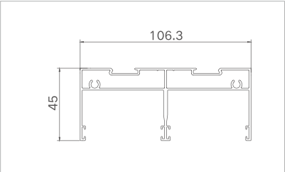
Model: XJ-ZTDM10615 ( Upper rail ) Thickness: 1.2mm Weight: 1.364kg/m
