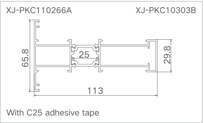
Model: XJ-DQPK110266 ( Middle column ) Thickness: 1.3mm Weight: 1.624kg/m
