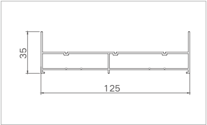
Model: XJ-FTLC12501 ( Outer frame ) Thickness: 1.3mm Weight: 1.134kg/m
