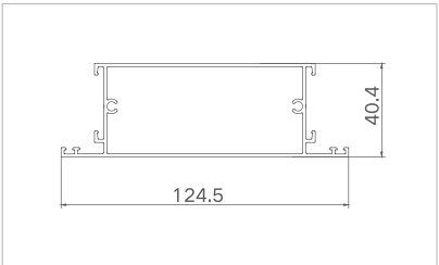
Model: XJ-FPKC4004 ( Middle column ) Thickness: 1.4mm Weight: 1.325kg/m
