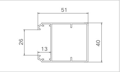
Model: XJ-PKM40200 ( Glass sash ) Thickness: 1.2mm Weight: 0.666kg/m
