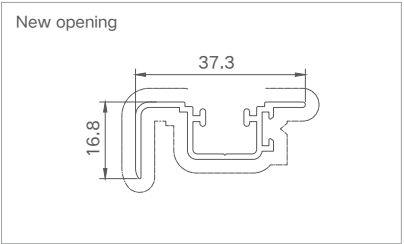
Model: XJ-DT13208D ( Double hook ) Thickness: 1.2mm Weight: 0.292kg/m
