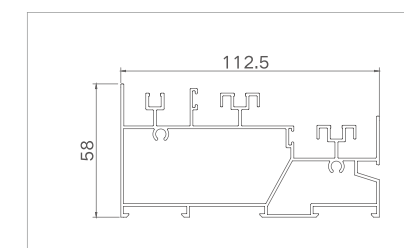
Model: XJ-FTLC11503 ( slide down )
