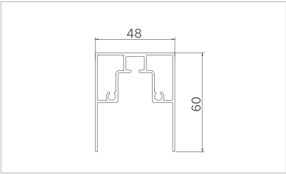
Model: XJ-TDM105239 ( Single upper rail ) Thickness: 1.3mm Weight: 1.002kg/m
