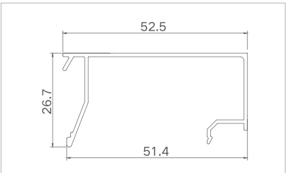
Model: XJ-PKC110270 ( Bending bead ) Thickness: 1.0mm Weight: 0.331kg/m
