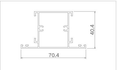
Model: XJ-FPKC4005 ( Small meddle column ) Thickness: 1.2mm Weight: 0.827kg/m
