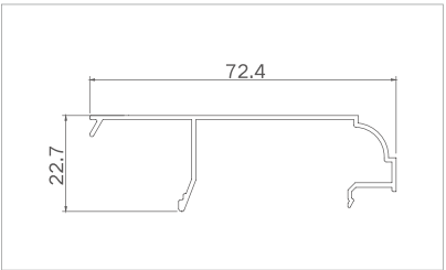
Model: XJ-PKC110269 ( Arc bead ) Thickness: 1.0mm Weight: 0.354kg/m
