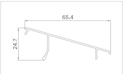
Model: XJ-PKC10893 Thickness: 1.1mm Weight: 0.304kg/m
