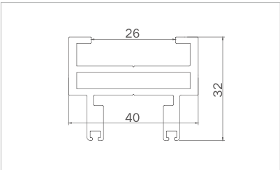
Model: XJ-TDM105231 ( Up and down horizontal ) Thickness: 2.0mm Weight: 0.967kg/m
