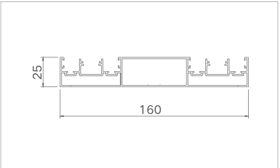
Model: XJ-ZTDM16006 ( three-rail frame ) Thickness: 1.2mm Weight: 1.731kg/m
