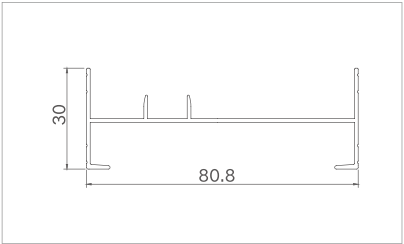
Model: XJ-TLC8001 Thickness: 1.1mm Weight: 0.488kg/m
