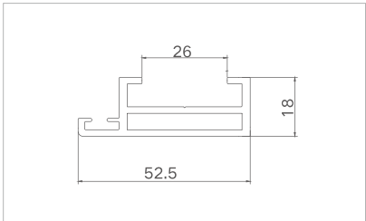
Model: XJ-TDM105232A ( Hook material ) Thickness: 2.0mm Weight: 0.775kg/m
