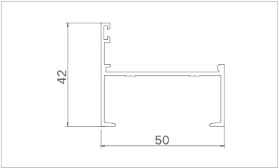
Model: XJ-PKC5017 Thickness: 1.4mm Weight: 0.52kg/m
