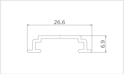
Model: XJ-TLC11505C ( Lock bar ) Thickness: 1.2mm Weight: 1.135kg/m
