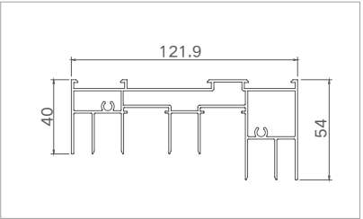
Model: XJ-FTLC12502 ( Slide up ) Thickness: 1.3mm Weight: 1.93kg/m
