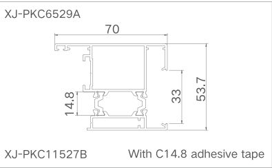
Model: XJ-PKC11527 ( Glass sash ) Thickness: 1.3mm Weight: 1.413kg/m
