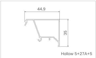
Model: XJ-PKC9577 ( Bead ) Thickness: 1.0mm Weight: 0.408kg/m
