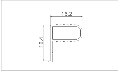
Model: XJ-XL516 Thickness: 1.0mm Weight: 0.14kg/m
