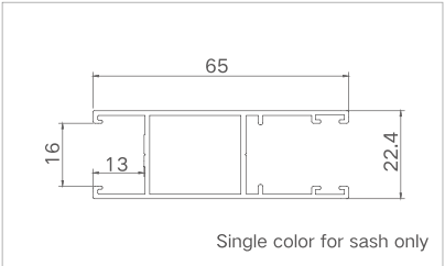
Model: XJ-TLC11507 ( Yarn sash ) Thickness: 1.2mm Weight: 0.635kg/m
