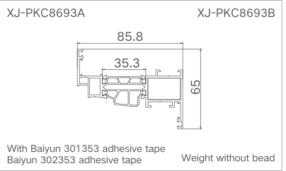
Model: XJ-DQPK8693 ( Glass sash ) Thickness: 1.75mm Weight: 1.609kg/m
