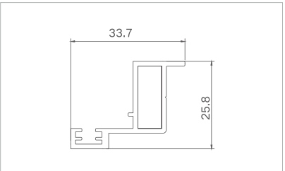
Model: XJ-PKC9576A ( Conversion frame ) Thickness: 1.4mm Weight: 0.348kg/m
