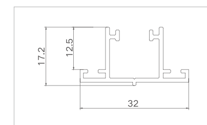
Model: XJ-FTLC11507 ( lock slots )
