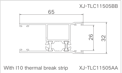
Model: XJ-DQTLC11505 ( Glass sash ) Thickness: 1.4mm Weight: 1.002kg/m
