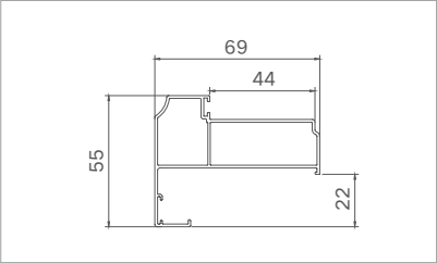
Model: XJ-PKM40201 ( front door casing ) Thickness: 1.15mm Weight: 0.819kg/m
