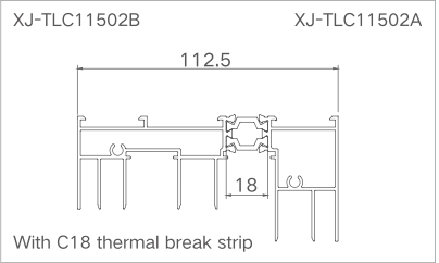
Model: XJ-DQTLC11502 ( Slide up ) Thickness: 1.3mm Weight: 1.999kg/m
