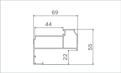
Model: XJ-PKM40202 ( back door casing ) Thickness: 1.15mm Weight: 0.819kg/m
