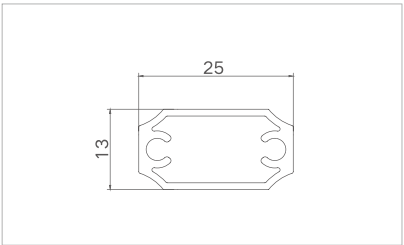
Model: XJ-XL496 ( Anti-theft grille ) Thickness: 1.1mm Weight: 0.261kg/m
