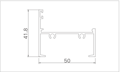
Model: XJ-PKC5018 Thickness: 1.4mm Weight: 0.57kg/m
