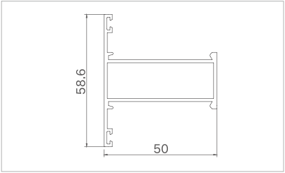
Model: XJ-PKC5020 Thickness: 1.4mm Weight: 0.76kg/m
