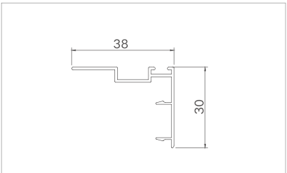
Model: XJ-TLC8038-A ( Hook ) Thickness: 1.0mm Weight: 0.24kg/m
