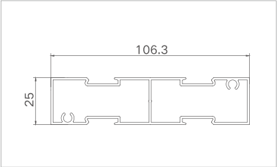
Model: XJ-ZTDM10612 Thickness: 1.2mm Weight: 1.094kg/m
