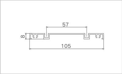
Model: XJ-TDM10534 ( track rail ) Thickness: 1.35mm Weight: 0.635kg/m
