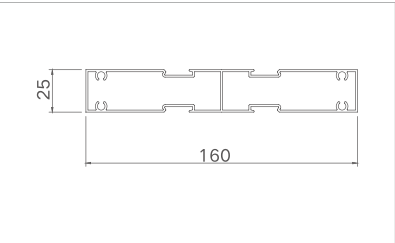
Model: XJ-ZTDM16009 ( three-rail middle column ) Thickness: 1.2mm Weight: 1.523kg/m
