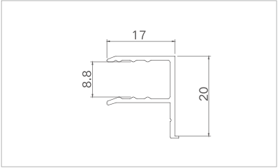
Model: XJ-XL515 Thickness: 1.2mm Weight: 0.161kg/m
