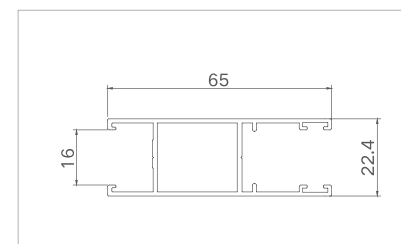
Model: XJ-TLC11507 ( Yarn sash )
