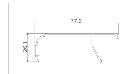
Model: XJ-TLC11509 ( circular arc bead )
